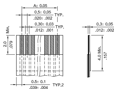
Accommodated FFC/FPC
