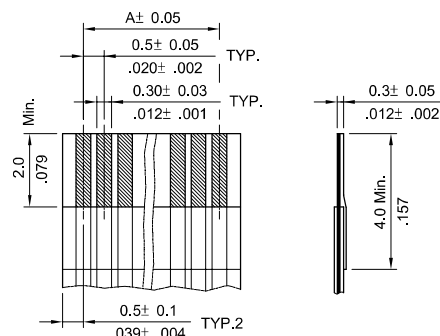
Accommodated FFC/FPC
