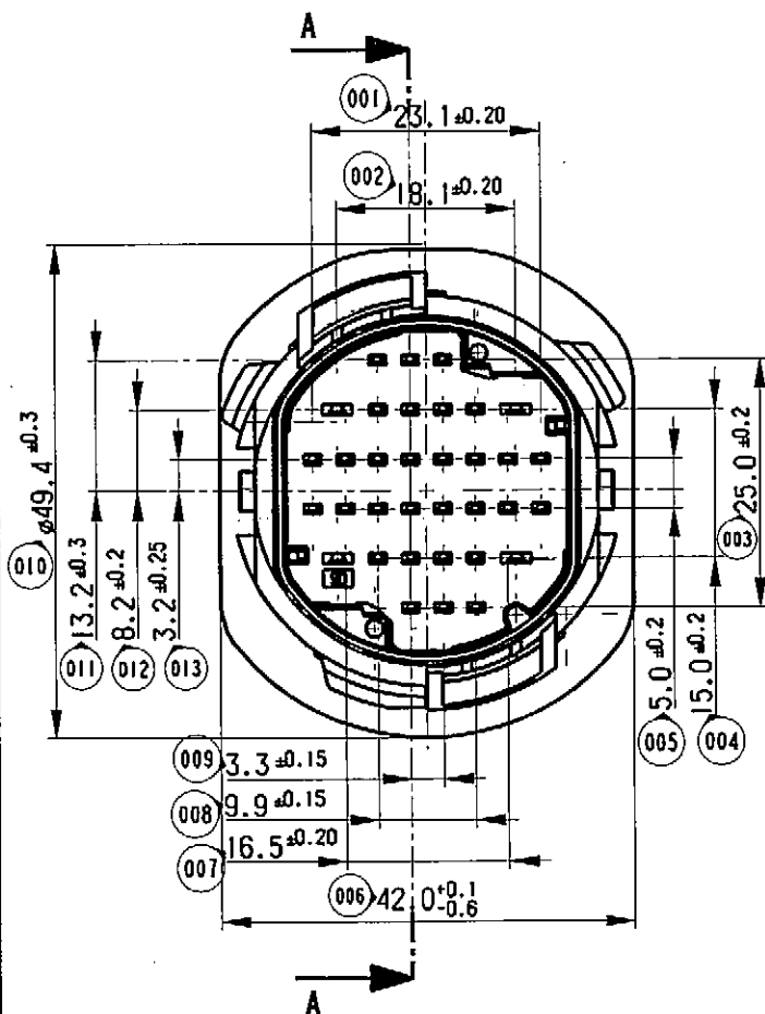
View "X" Scale 2:1
