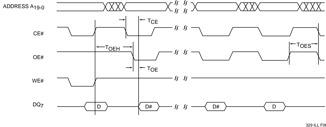
FIGURE 6: DATA# POLLING TIMING DIAGRAM
